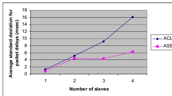
Figure 4c. Average std deviation in delay for ACL and ASB.
