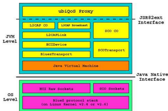
Figure 3. Architecture of the JSR82ext protocol stack.
