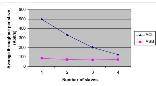
Figure 4a. Average throughput per slave for ACL and ASB.
