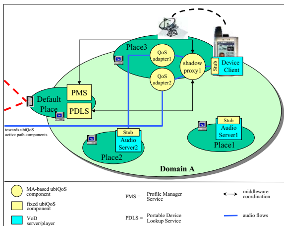
Figure 2. The ubiQoS middleware components in one domain.
